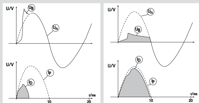
Current limiting DX 3 MCB
